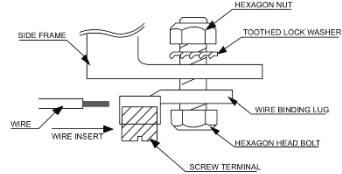
Figure 3. Example of acceptable ground connection
