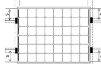
Figure 2. Clamping on Shorter Frame
