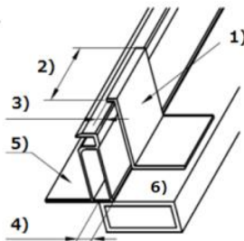
Figure1. Clips (Clamps) requirement
