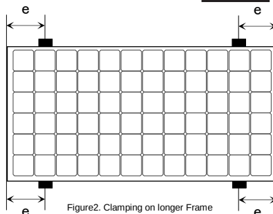
Figure2. Clamping on longer Frame 300 mm < e < 400 mm e : span from module corner to clip center
