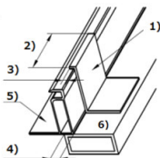
Schéma 1. Conditions requises - Clips (pattes de fixation)
