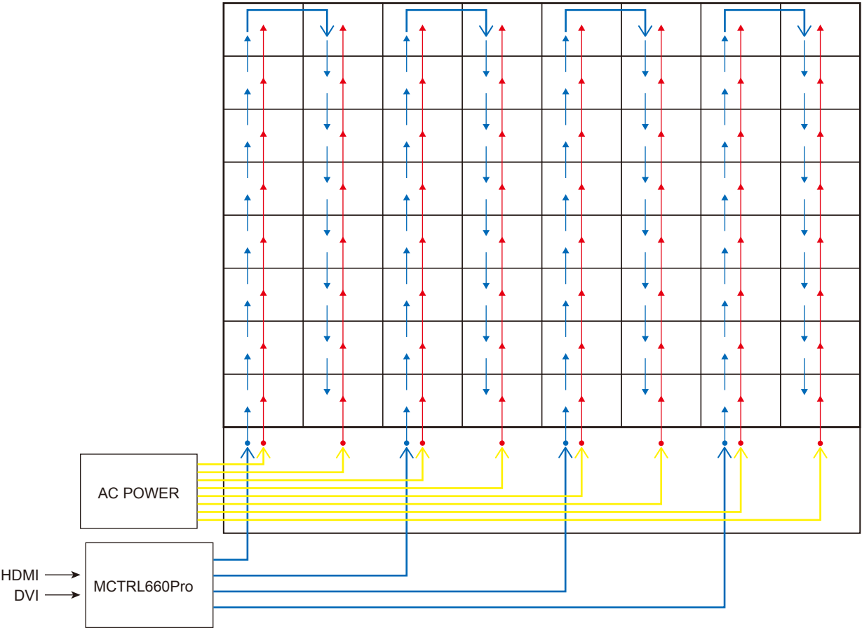
8 x 8 frame set (2.5 mm pitch, 3.8 mm pitch)
