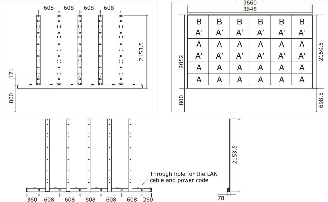
6 x 6 frame set (0.9 mm pitch)
