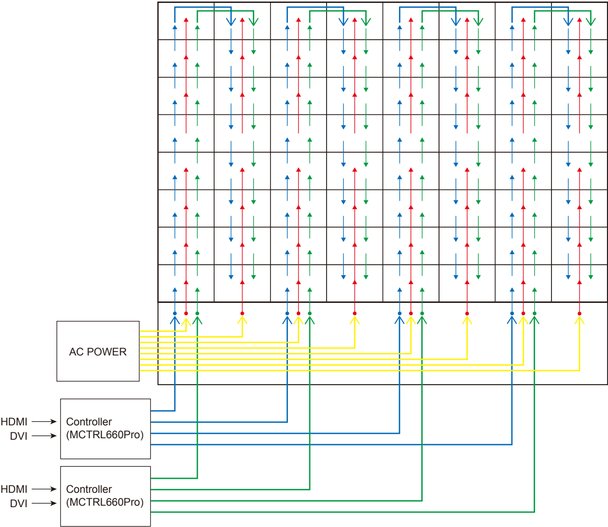
8 x 8 frame set (2.5 mm pitch, 3.8 mm pitch)
