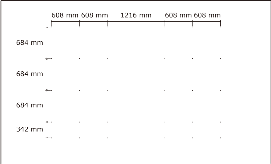
Anchor points positions: 8 x 8 frame set
