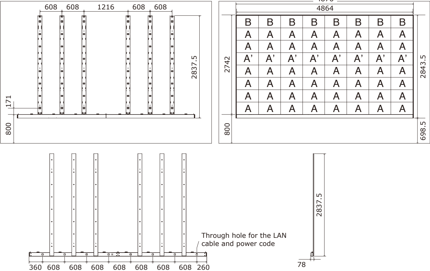
8 x 8 frame set (1.2 mm pitch)
