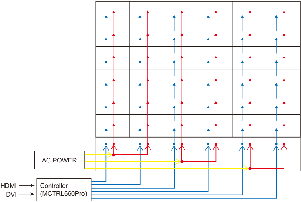
6 x 6 frame set (1.9 mm pitch)
