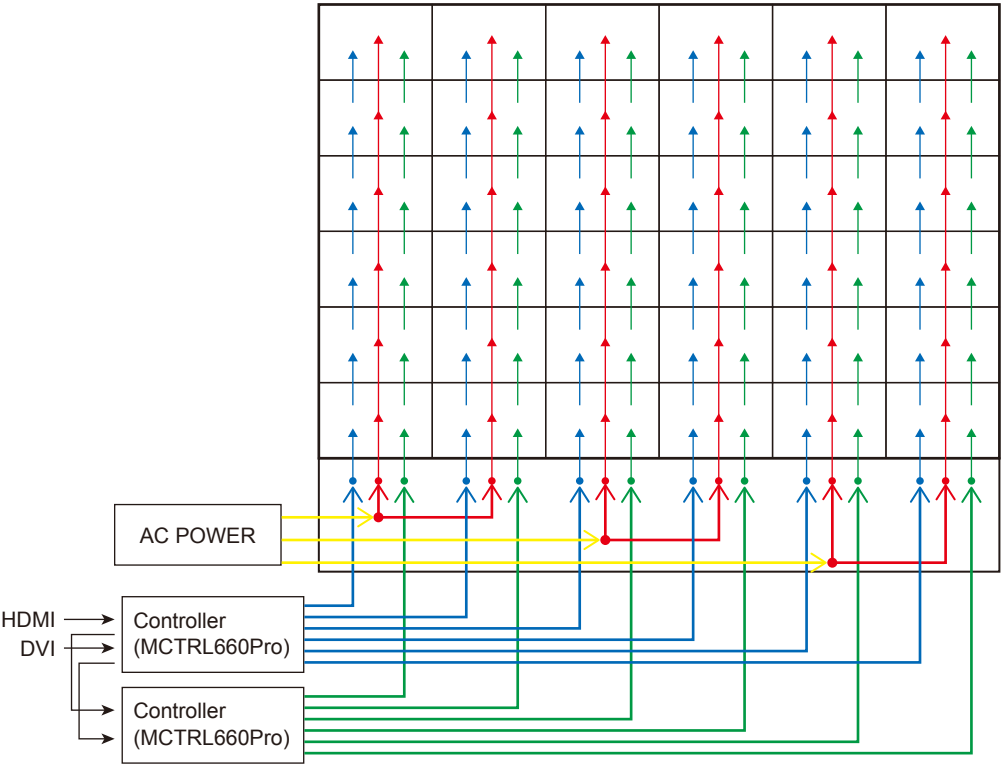
6 x 6 frame set (1.9 mm pitch)
