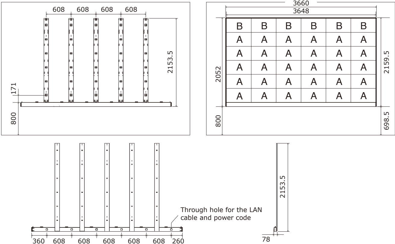
6 x 6 frame set (1.9 mm pitch)
