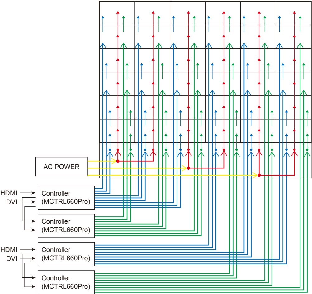
6 x 6 frame set (0.9 mm pitch)
