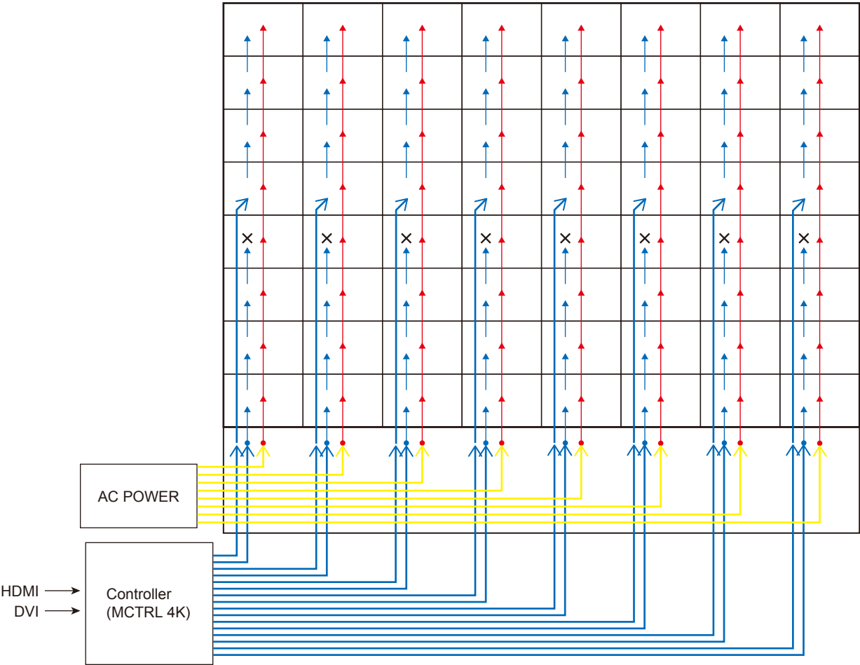
8 x 8 frame set (1.2 mm pitch)
