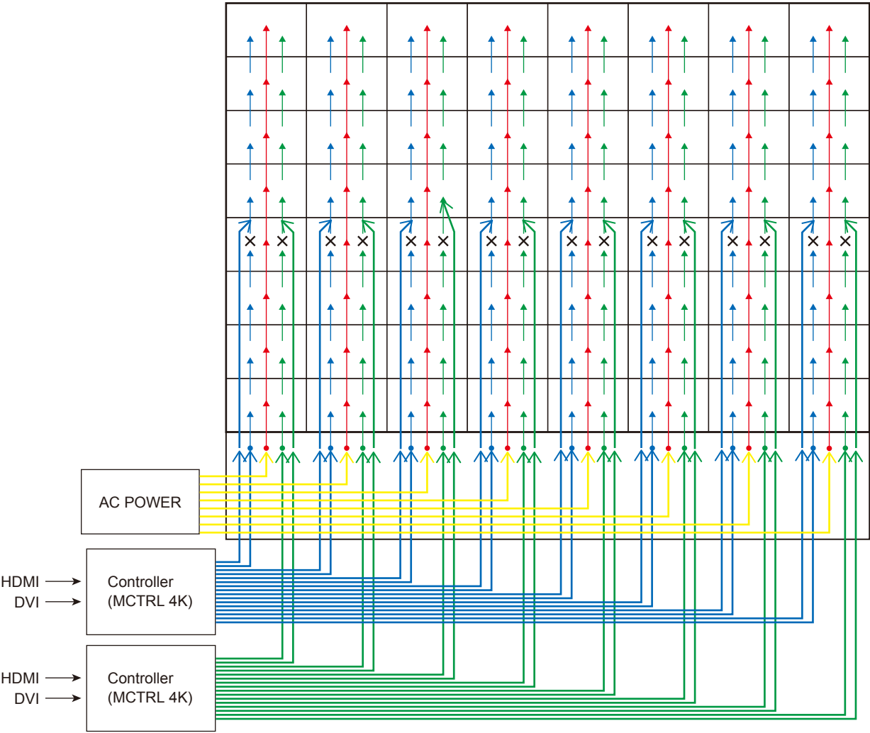
8 x 8 frame set (1.2 mm pitch)
