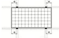
Figure2. Clamping on longer Frame
