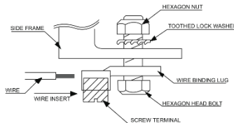
Figure 3. Example of acceptable ground connection
