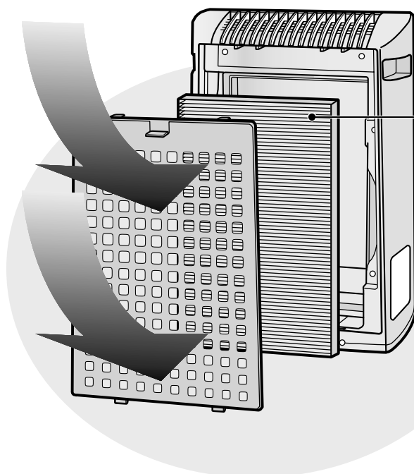
Dust Collection / Deodorizing Filter
